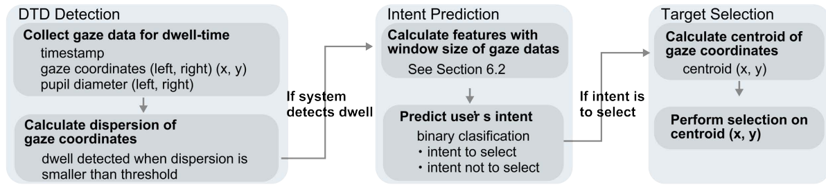
Fig. 1. Overview of DTD-ML selection.
